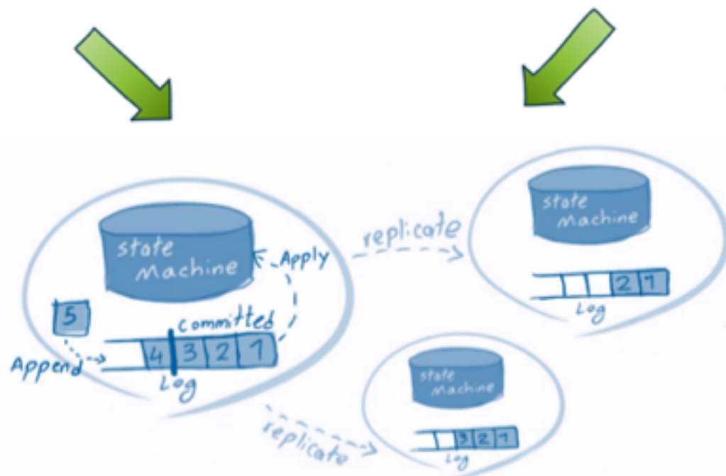
统一抽象为 ReplicatedStateMachine (RSM)
